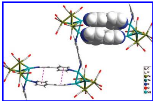
Figure 2. Intramolecular \pi – \pi interactions of polymer 2 .
