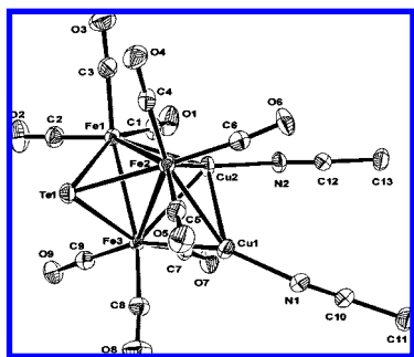
Figure 3. ORTEP diagram of 3 , showing 30% probability thermal ellipsoids. Selected bond distances (Å) and angles (deg): Te(1)–Fe(1) 2.485(1), Te(1)–Fe(2) 2.483(9), Te(1)–Fe(3) 2.489(1), Fe(1)–Fe(2) 2.742(1), Fe(1)–Fe(3) 2.695(1), Fe(2)–Fe(3) 2.801(1), Cu(2)–Fe(1) 2.471(1), Cu(2)–Fe(2) 2.529(1), Cu(2)–Fe(3) 2.595(1), Cu(1)–Fe(2) 2.535(1), Cu(1)–Fe(3) 2.487(1), Cu(1)–Cu(2) 2.605(1), Cu(1)–N(1) 1.918(7), Cu(2)–N(2) 1.940(6), N(1)–C(10)–C(11) 179.4(8), N(2)–C(12)–C(13) 178.3(7).
