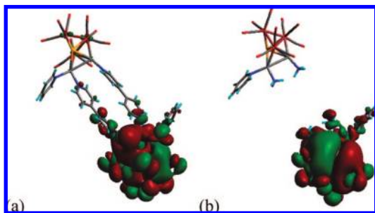
Figure 4. Spatial plots of HOMO of (a) H_2\{[TeFe_3(CO)_9Cu_2](\mu-4,4'-dipyridyl)_{1.5}\}_2 ( 2a ) and (b) H_2\{[TeFe_3(CO)_9Cu_2(NH_3)_2](\mu-4,4'-dipyridyl)_{0.5}\}_2 ( 2a' ) (isovalue = 0.004).
