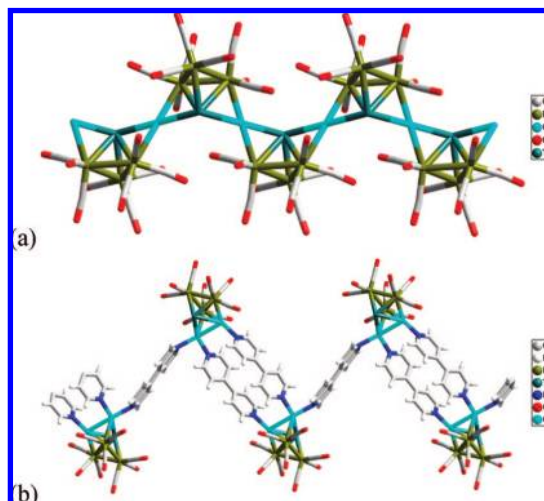
Figure 1. Portion of the zigzag chains of polymers (a) 1 and (b) 2 .
